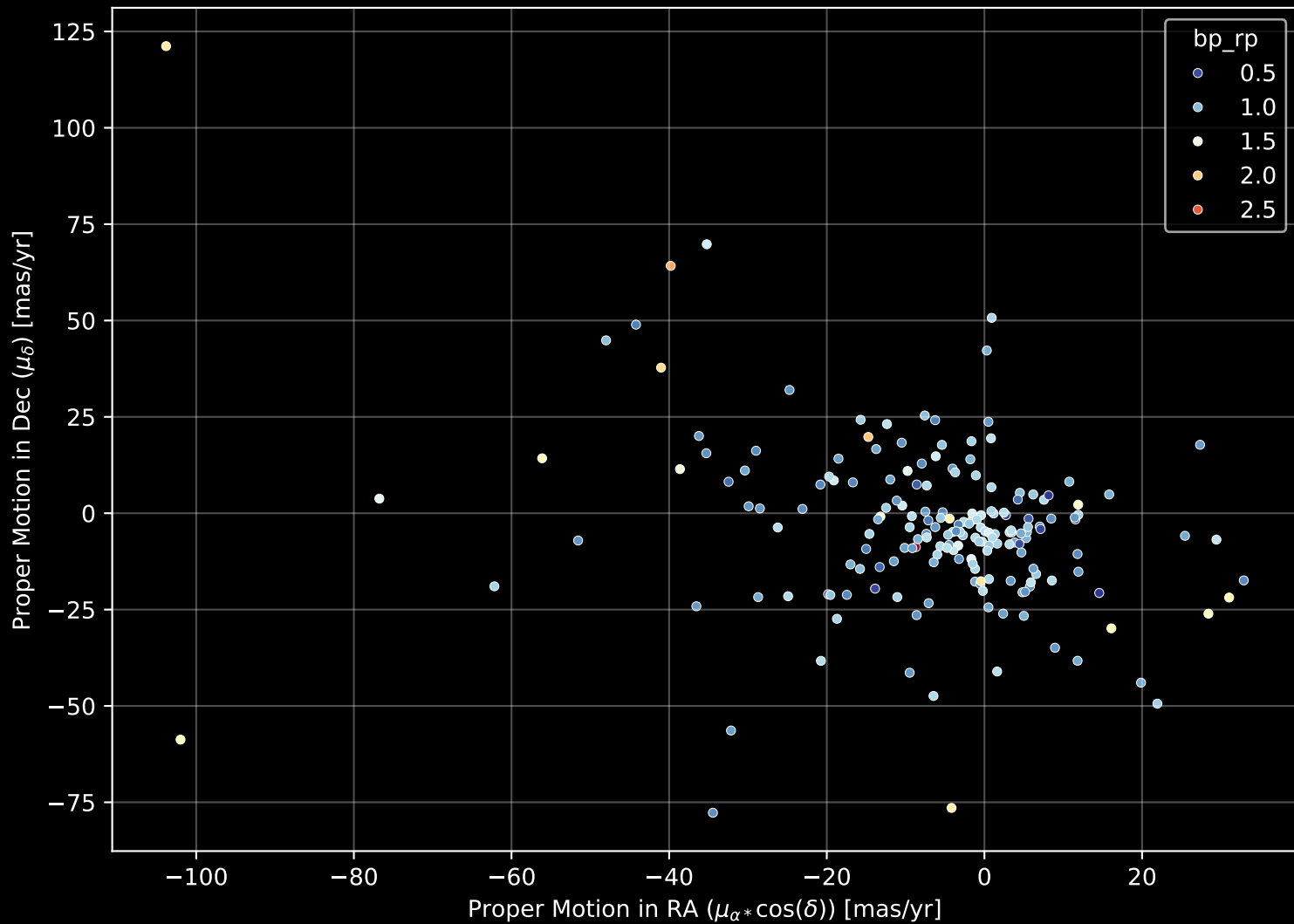
APOGEE DR17 Field: [053+38_MGA] Proper Motion Diagram (n= 188)
