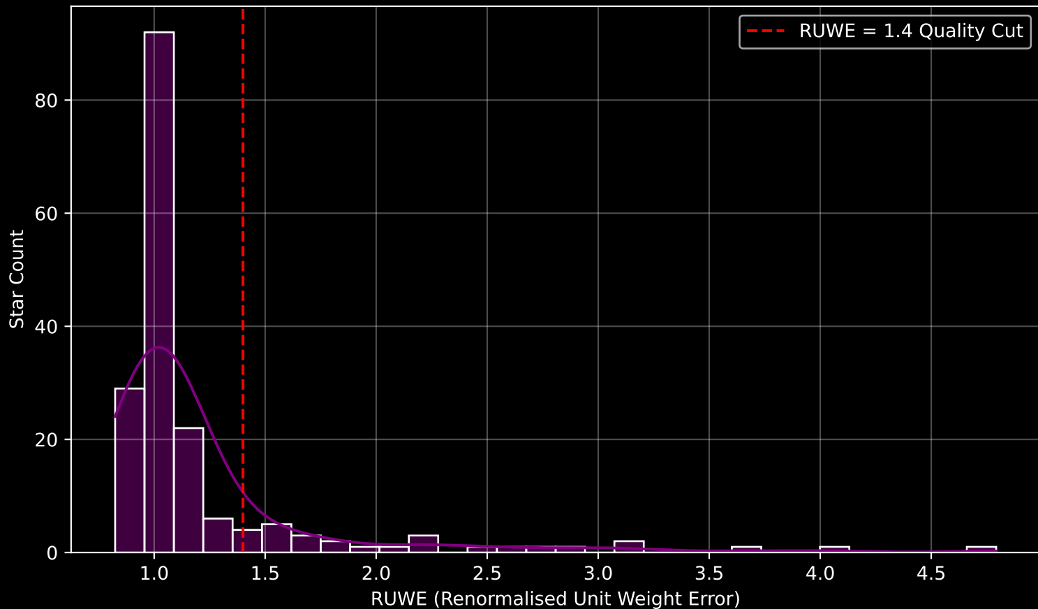
GAPOGEE DR17 Field [053+38_MGA] RUWE Distribution (n= 177)
