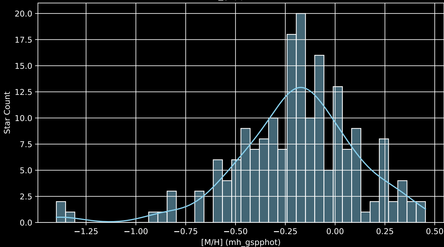
APOGEE DR17 Field: [053+38_MGA [M/H] (mh_gspphot) (n= 187)
