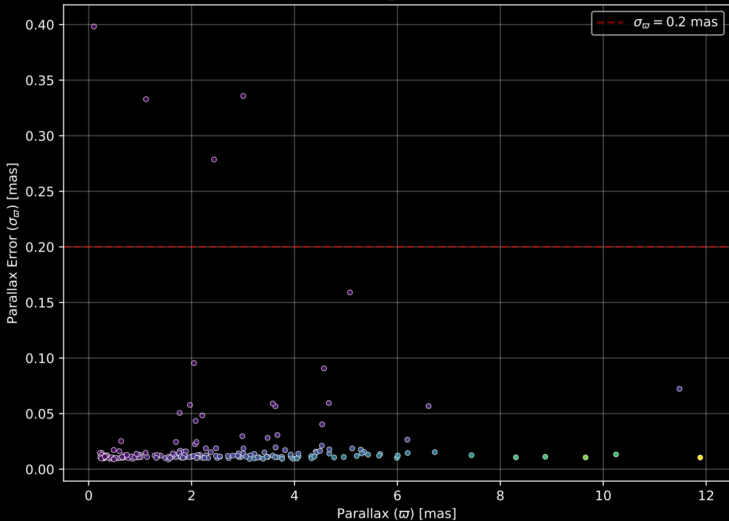
APOGEE DR17 Field: [053+38_MGA] Parallax Quality (n= 188)
