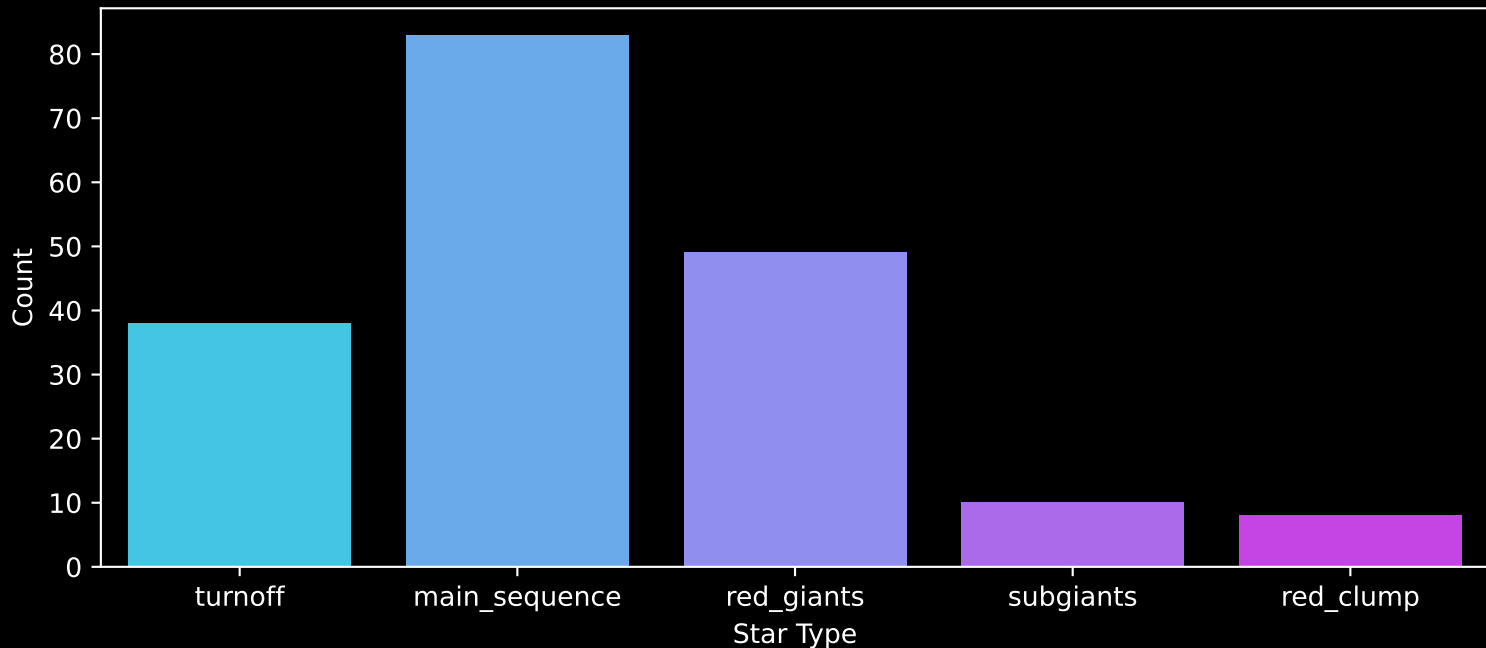
APOGEE DR17 Field: [053+38_MGA] Count plot of Star Type
