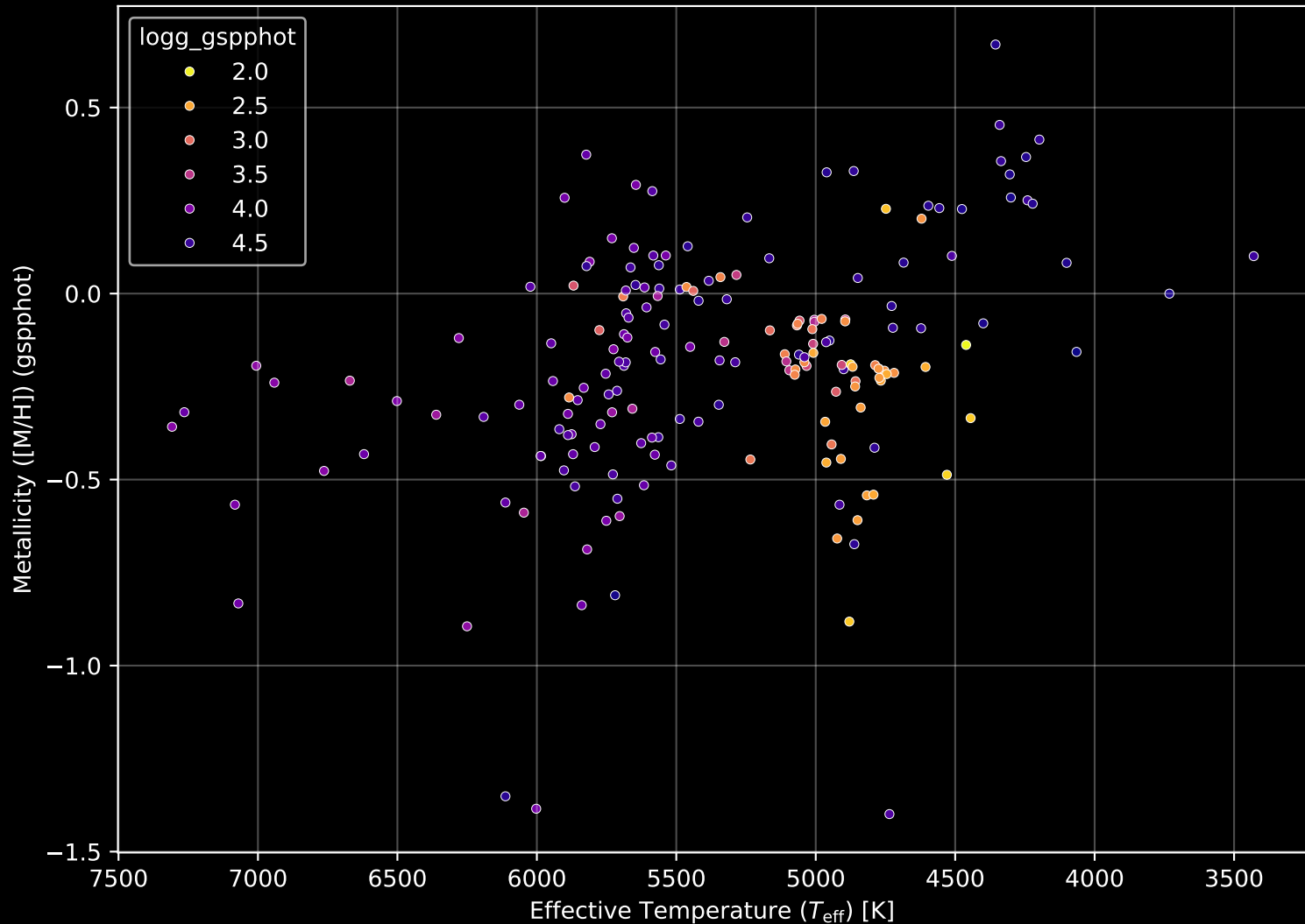
APOGEE DR17 Field: [053+38_MGA] Stellar Population Parameters (n= 188)
