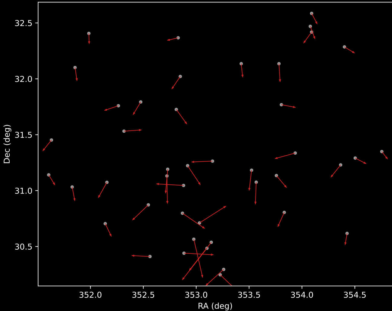
APOGEE DR17 Cluster 6 Proper Motion Vectors (n=44)
